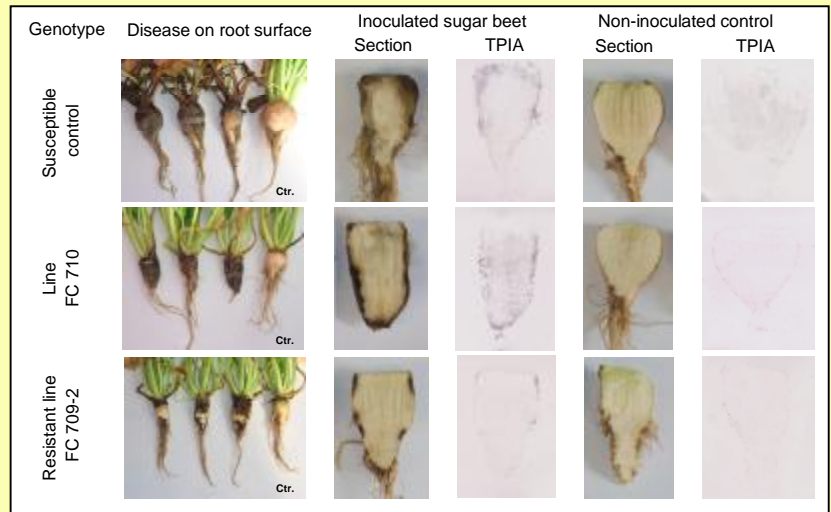
Fig. 2: Disease severity of sugar beet genotypes inoculated with R. solani isolates as determined on root surface, longitudinal sections and TPIA. Ctr: non-inoculated control.
