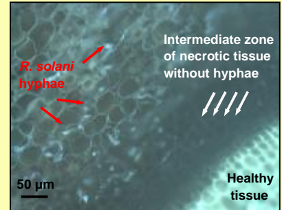
Fig. 1: Transverse section of R. solani infected sugar beet root (Calcofluor White)
