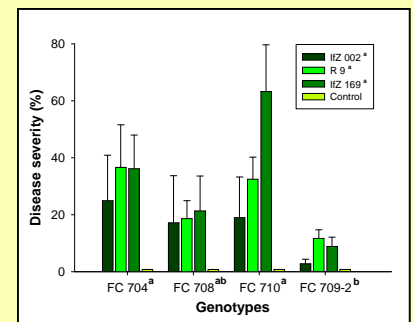
Fig. 4: Disease severity of sugar beet genotypes inoculated with R. solani isolates
