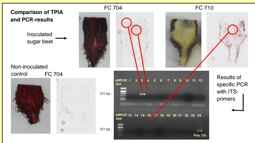
Fig. 3: Longitudinal sections of inoculated resp. control sugar beet, tissue print of same sections and results of specific PCR. Lane 24: positive control.
